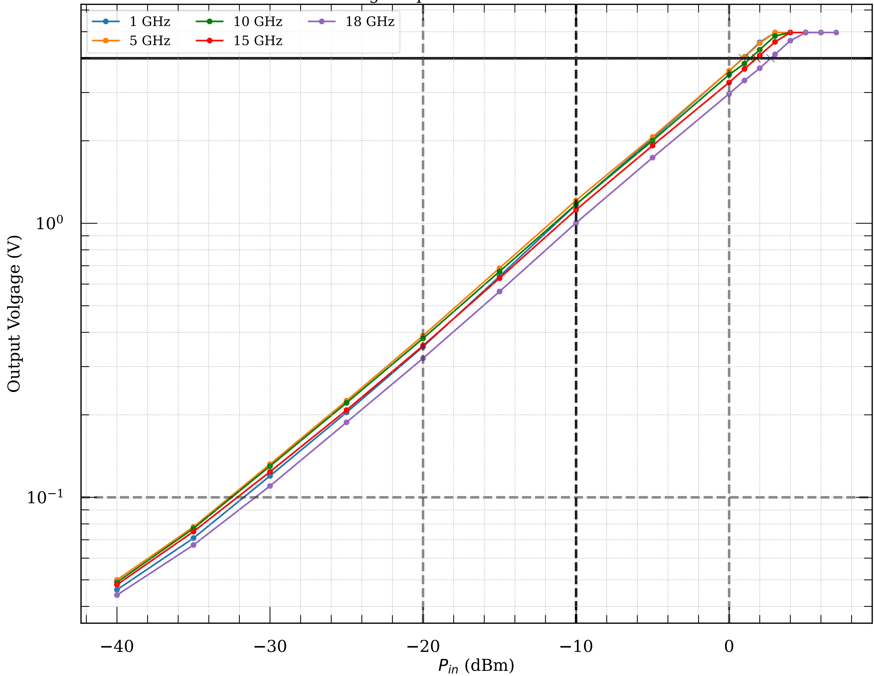
Measured voltage-to-power curve of detector module047
